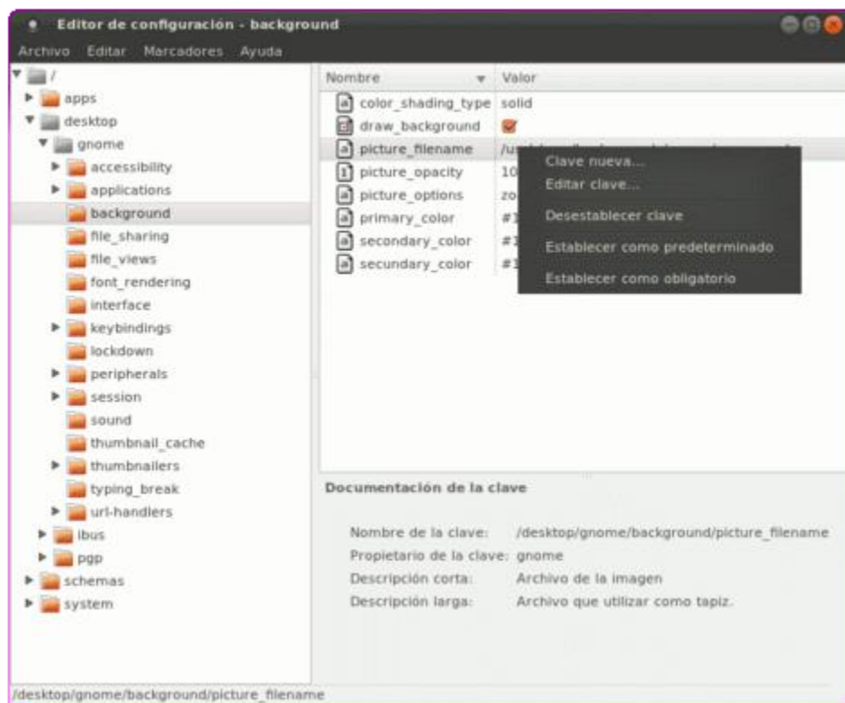
GConf-editor.
